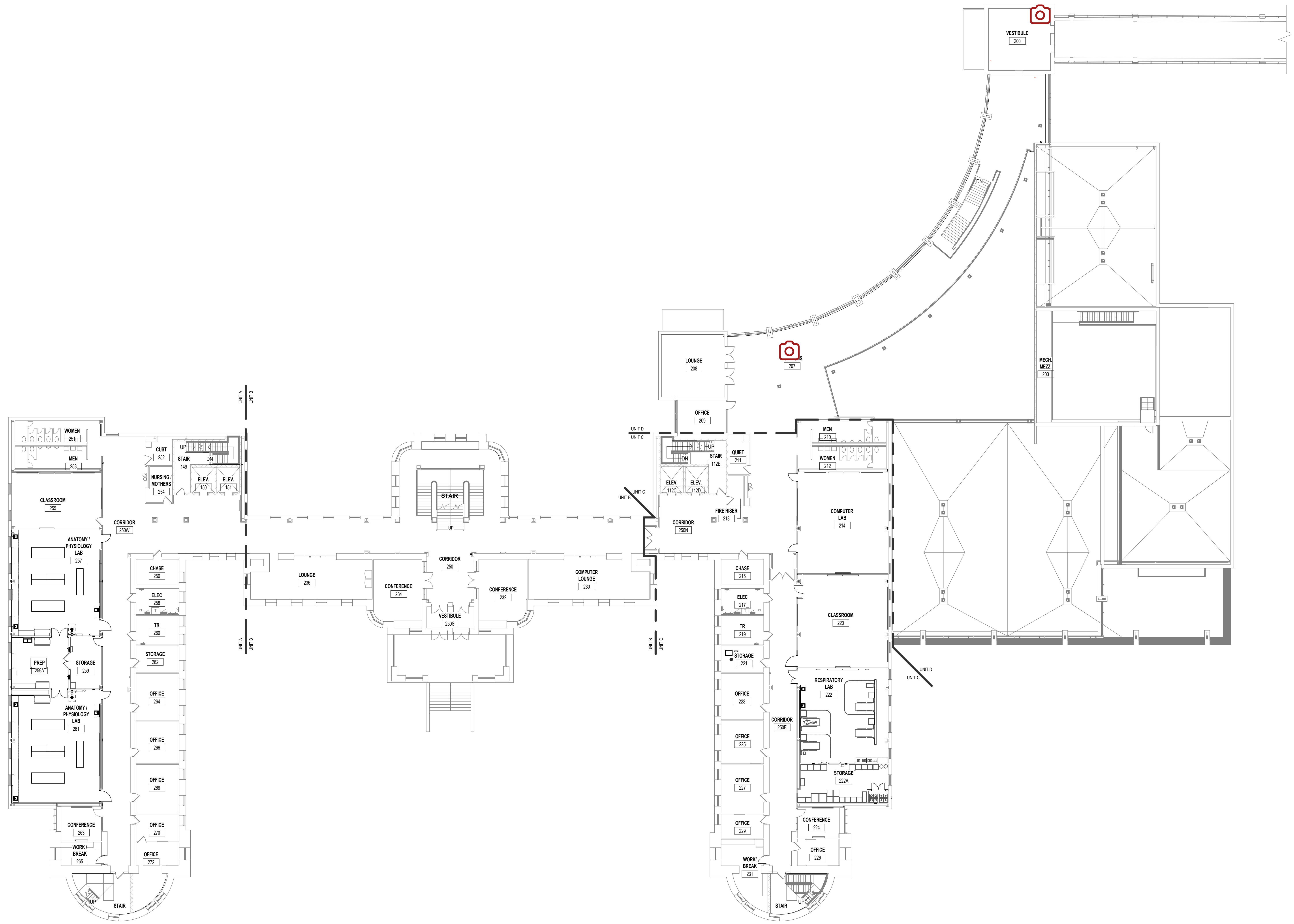
↑ SECOND FLOOR OVERALL PLAN 1/16" = 1'-0"
